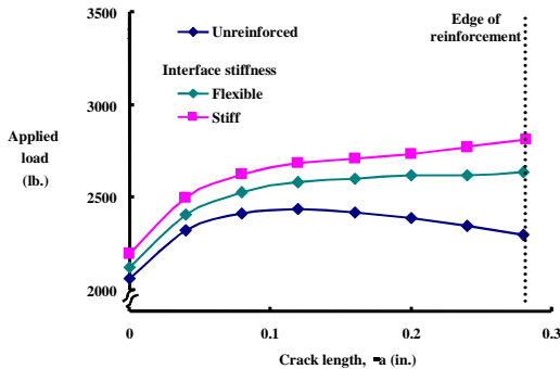
Figure 13. Predicted effect of interface stiffness on fracture response (reinforcement width = 0.50", reinforcement thickness = 40 present).
