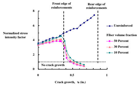
Figure 8. Predicted effect of reinforcement stiffness on fatigue crack growth (reinforcement width = 0.5", reinforcement thickness = 40 percent, flexible interface).
